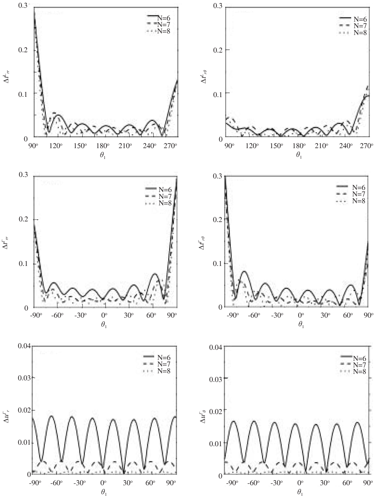
Fig. A-1 Stress residual and displacement residuals ( \theta = 45^\circ , \eta = 1.0 )
