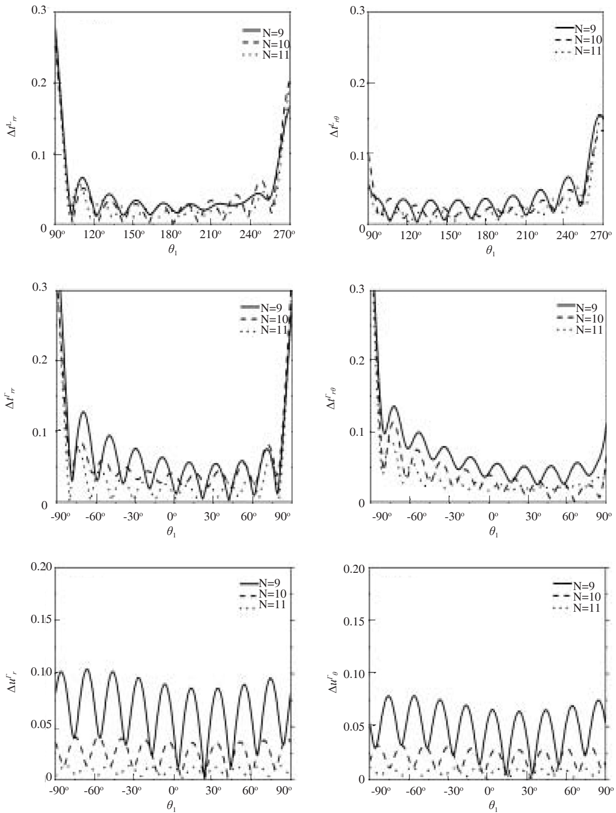
Fig. A-2 Stress residual and displacement residuals ( \theta_\alpha=45^\circ , \eta=3.0 )
